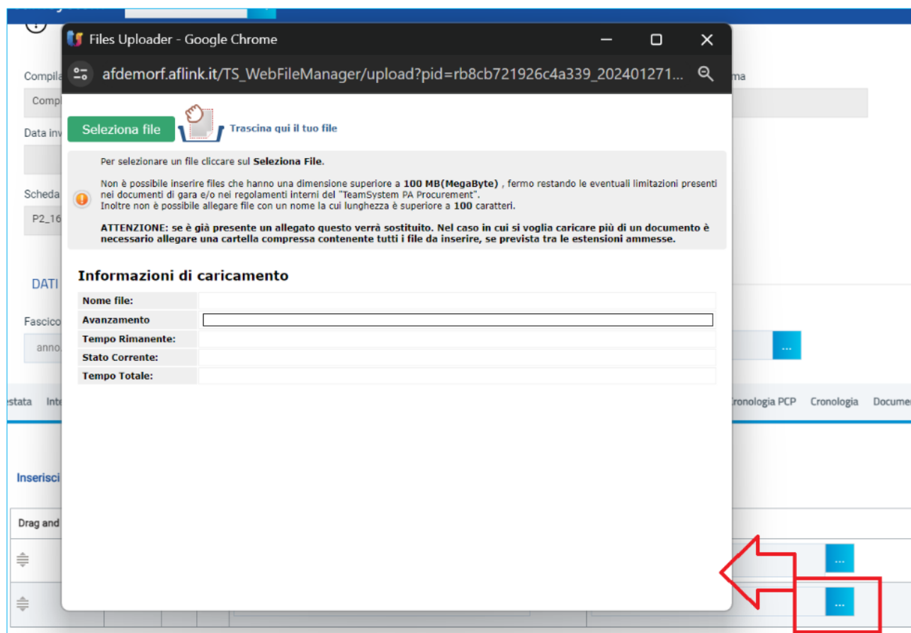
Figura 1 - Upload file
